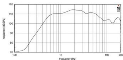
FREQUENCY RESPONSE MEASURED WITH 2.83 V INPUT ON AXIS AT 1 METER DISTANCE FROM THROAT OF XQ2054C HORN. IMPEDANCE MEASURED ON SAME HORN
